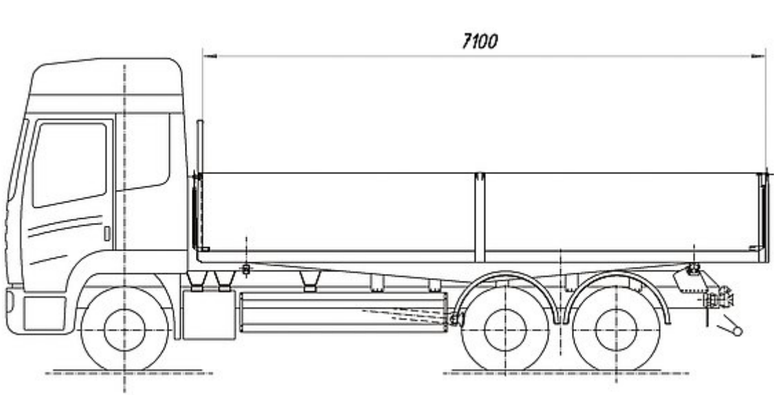
3-way tipper body on 3-axle truck - long-haul transport
