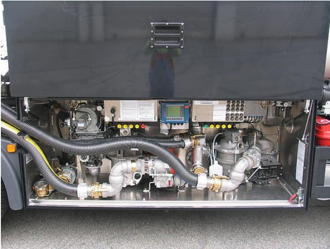
Fittings cabinet with parallel sliding cabinet door
