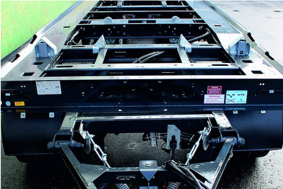
Adjustable stops at front for various container lengths
