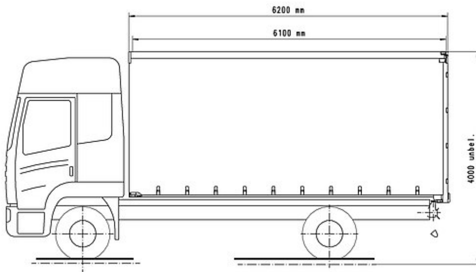
OPTIONAL: Variable load securing via bolt-on lashing systems, such as: airline lashing rail
